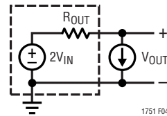
Figure 4. Equivalent Open-Loop Circuit
