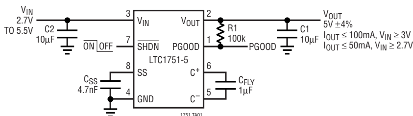
Regulated 5V Output from a 2.7V to 5.5V Input
