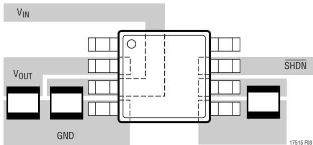
Figure 6. Recommended Layout
