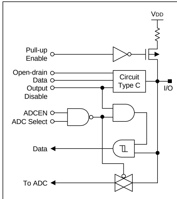
Figure 1-6. Pin Circuit Type F-16A
