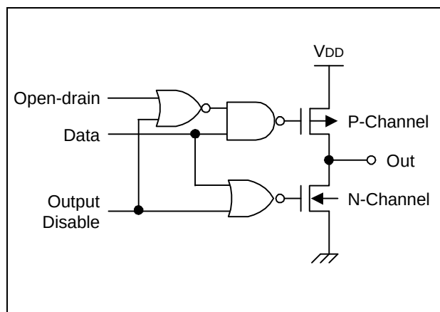
Figure 1-4. Pin Circuit Type C
