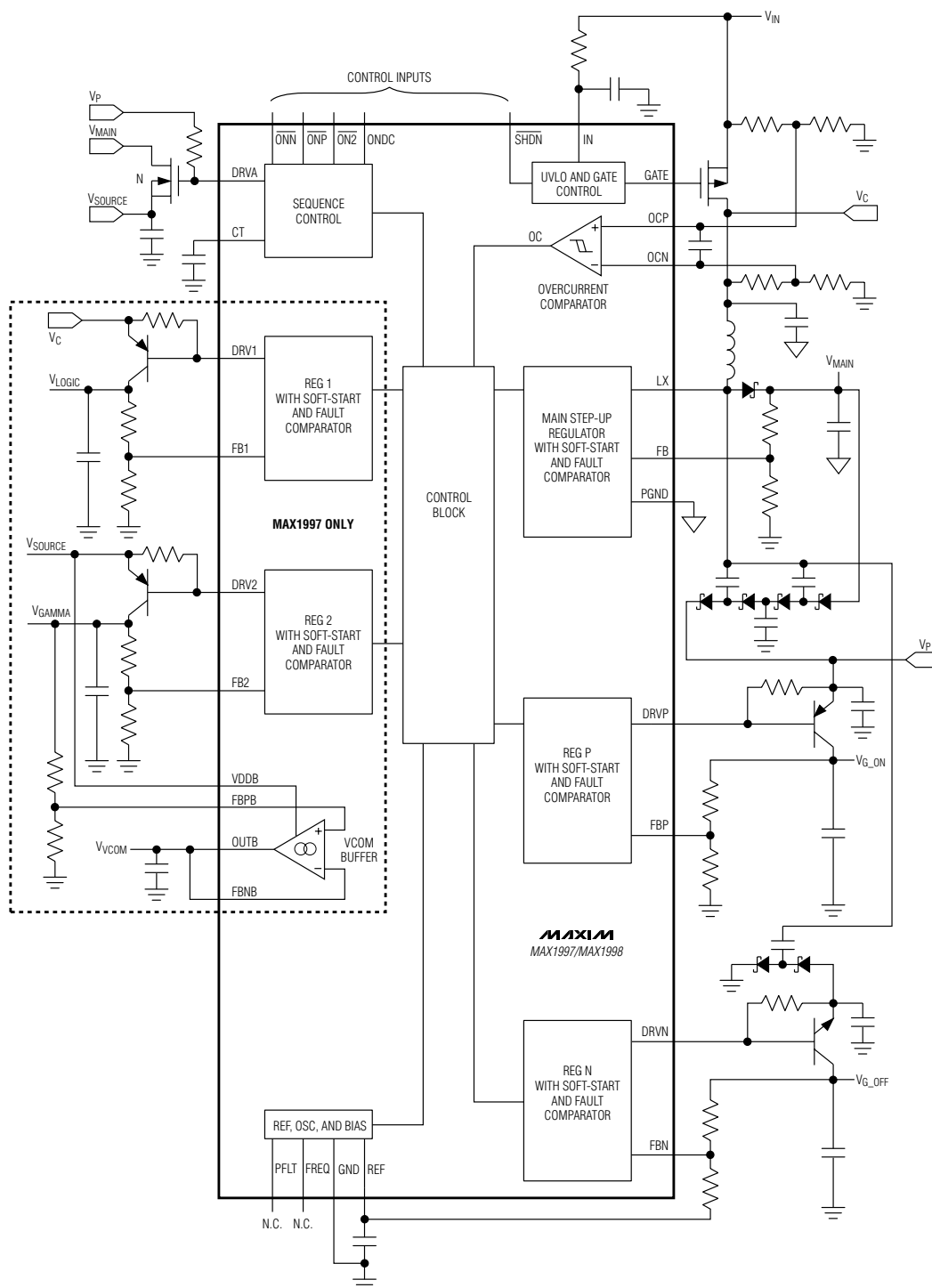
Figure 2. System Functional Diagram
