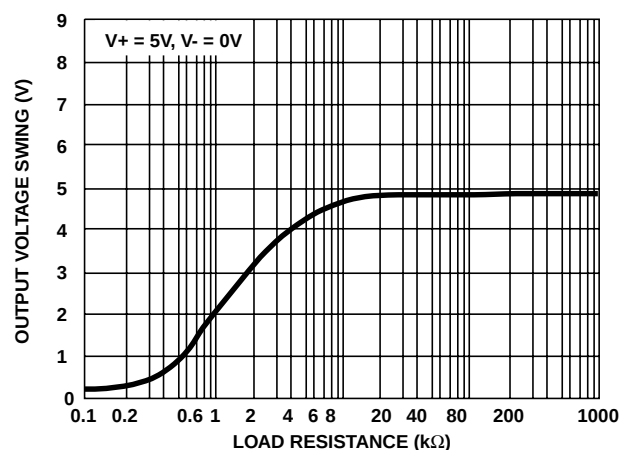
FIGURE 20. OUTPUT SWING vs LOAD RESISTANCE
