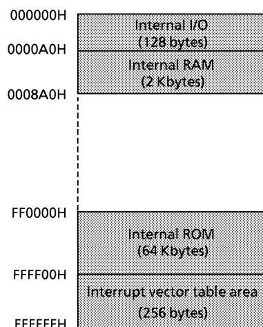
Memory map of TMP93CS20
