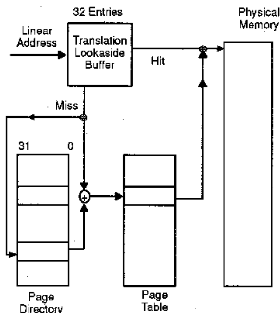
Figure 4-23 Translation Lookaside Buffer
