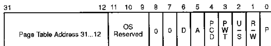
Figure 4-21 Page Directory Entry (Points to Page Table)
