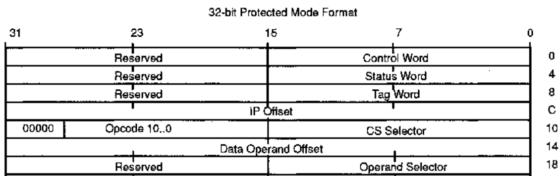
Figure 2-10 Protected Mode FPU Instruction and Data Pointer Image In Memory, 32-Bit Format
