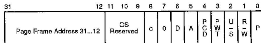
Figure 4-22 Page Table Entry (Points to Page)
