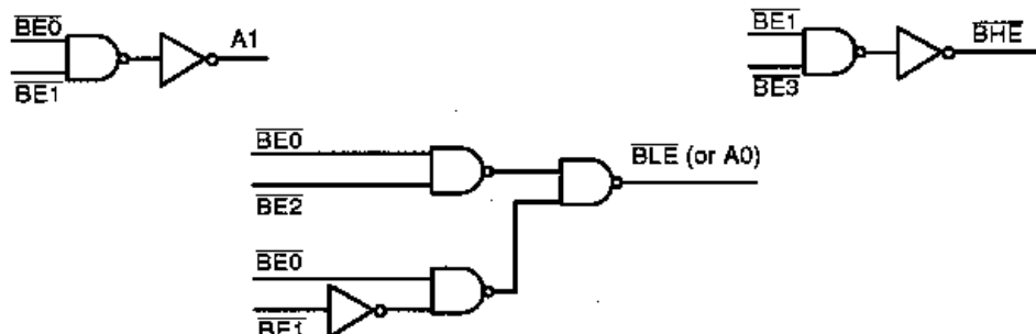
Figure 7-5 Logic to Generate A1, \overline{\text{BHE}} , and \overline{\text{BLE}} for 16-Bit Buses
