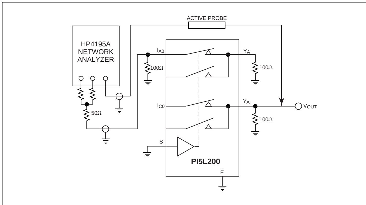
Figure 5. Off Isolation
