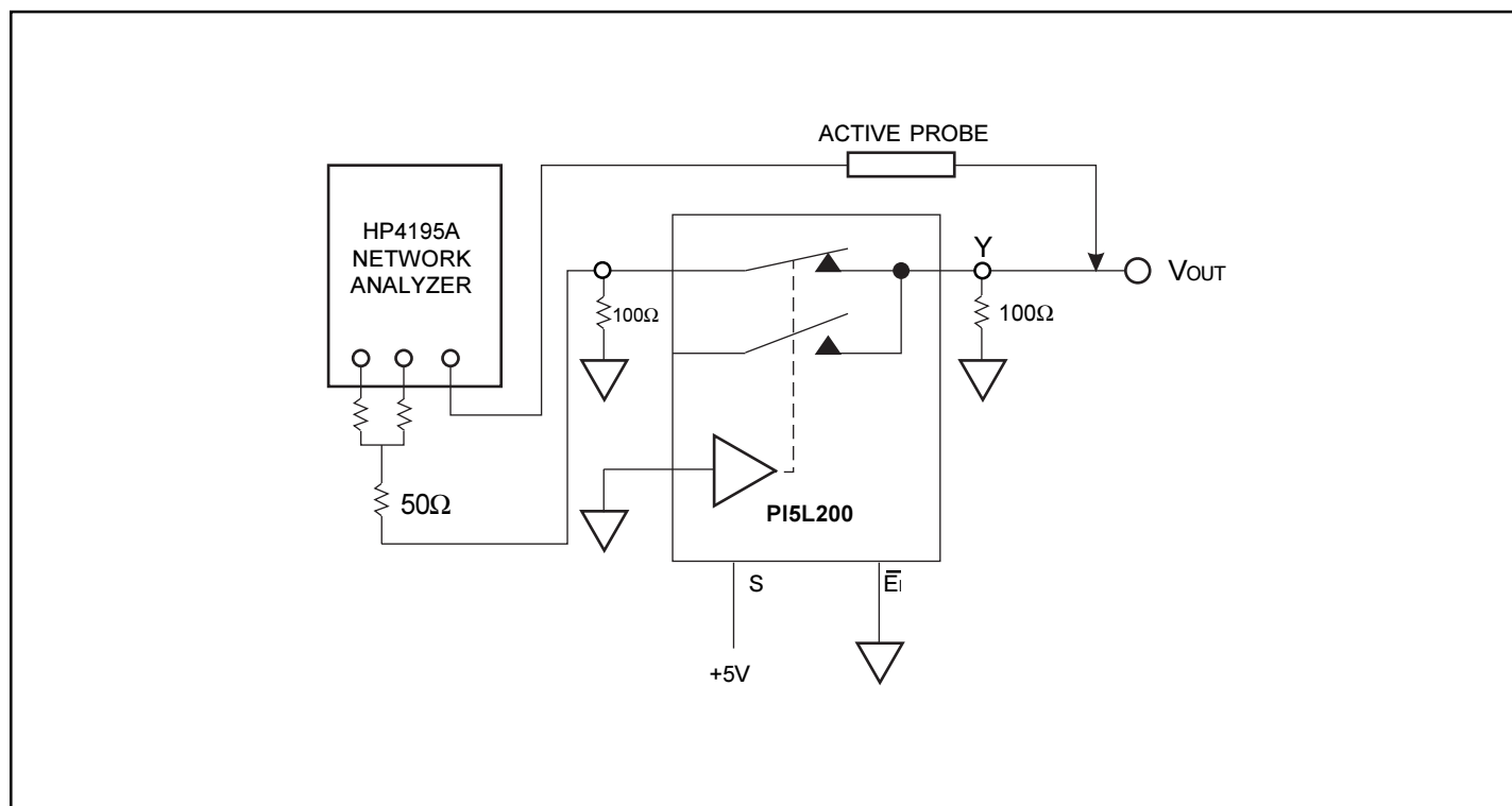
Figure3. Bandwidth
