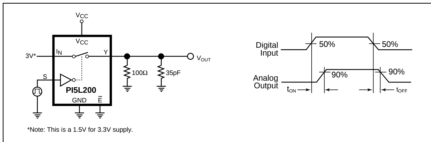
Figure2. Switching Time
