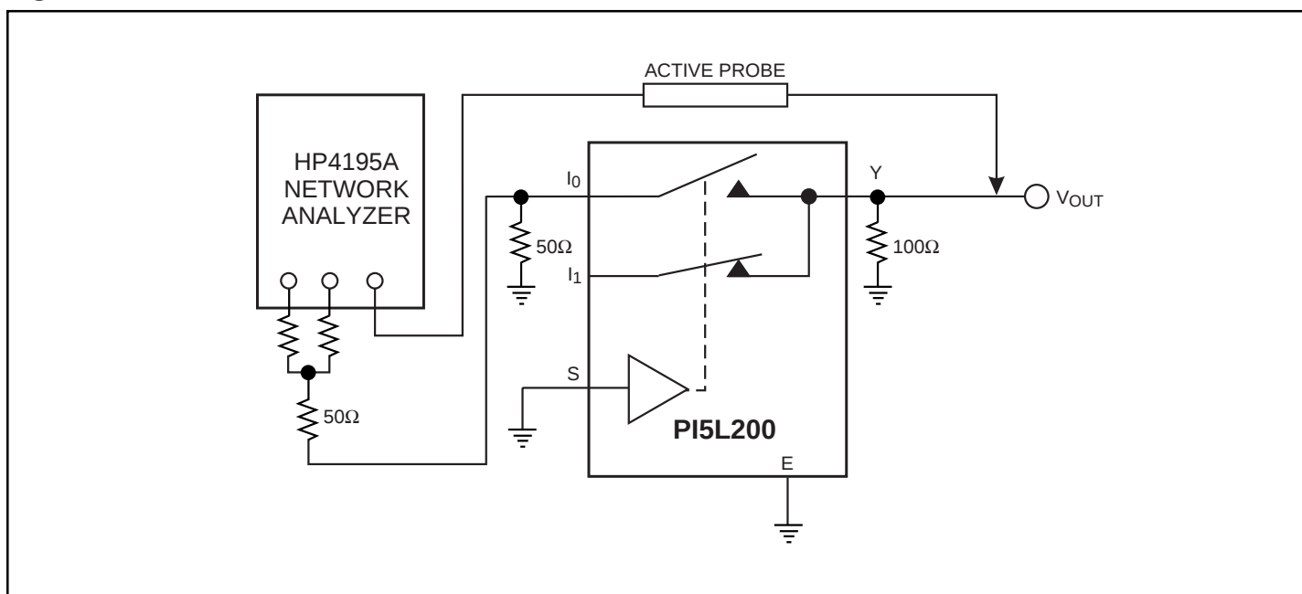
Figure 5. Off Isolation
