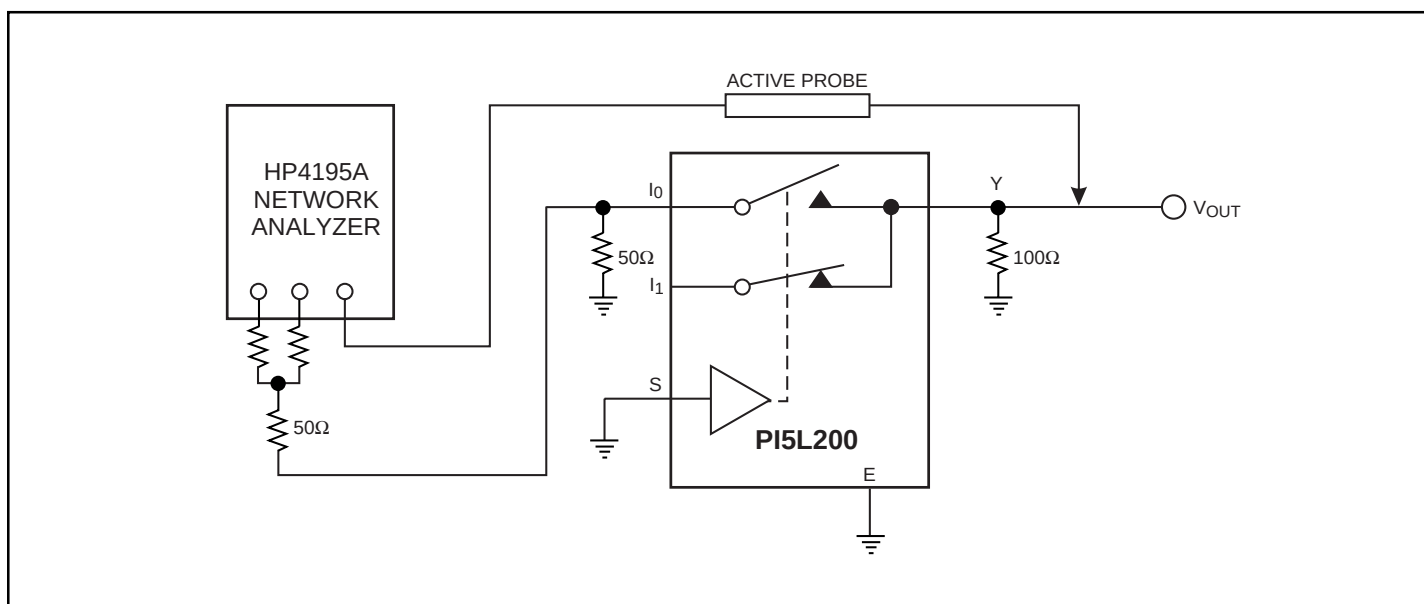
Figure 5. Off Isolation
