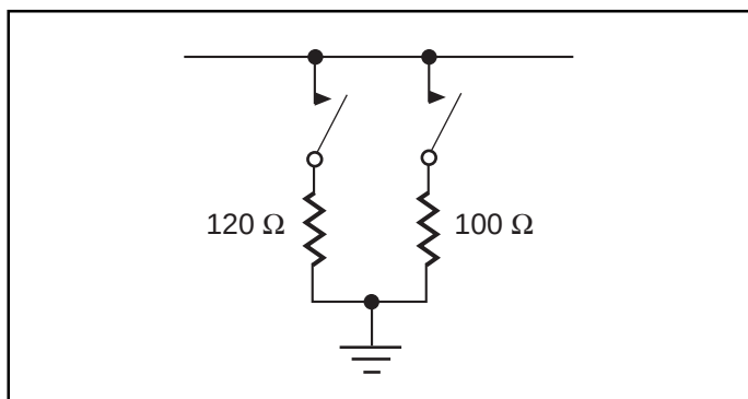
Figure 1c. Line Termination
