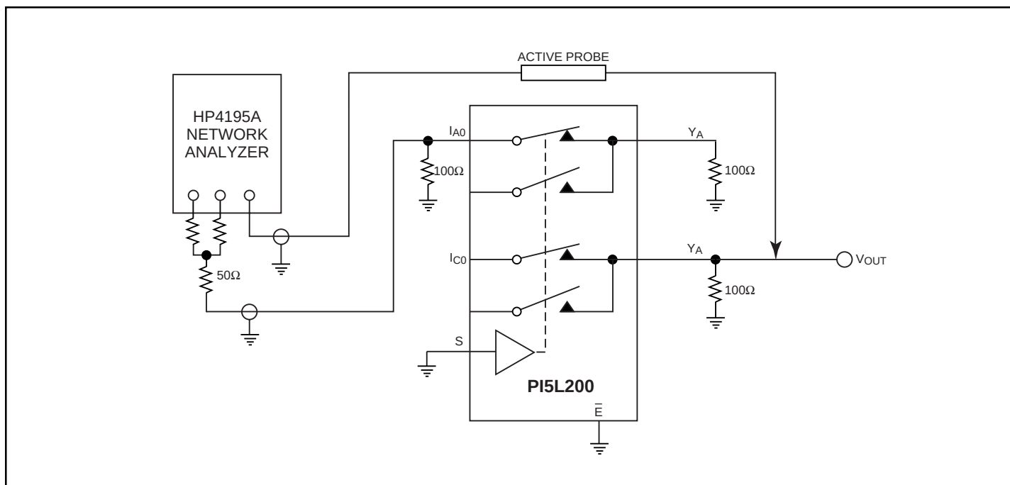
Figure 4. Crosstalk
