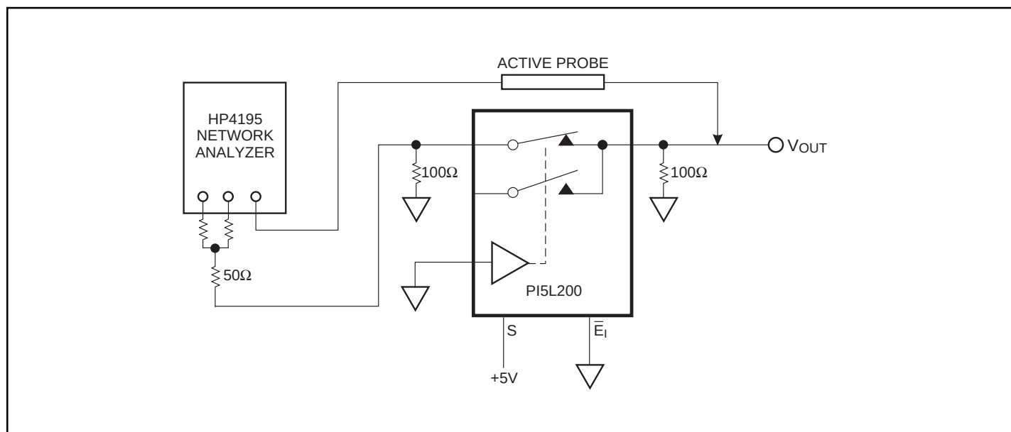
Figure 3. Bandwidth
