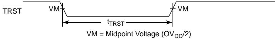
Figure 13. \overline{TRST} Timing Diagram
