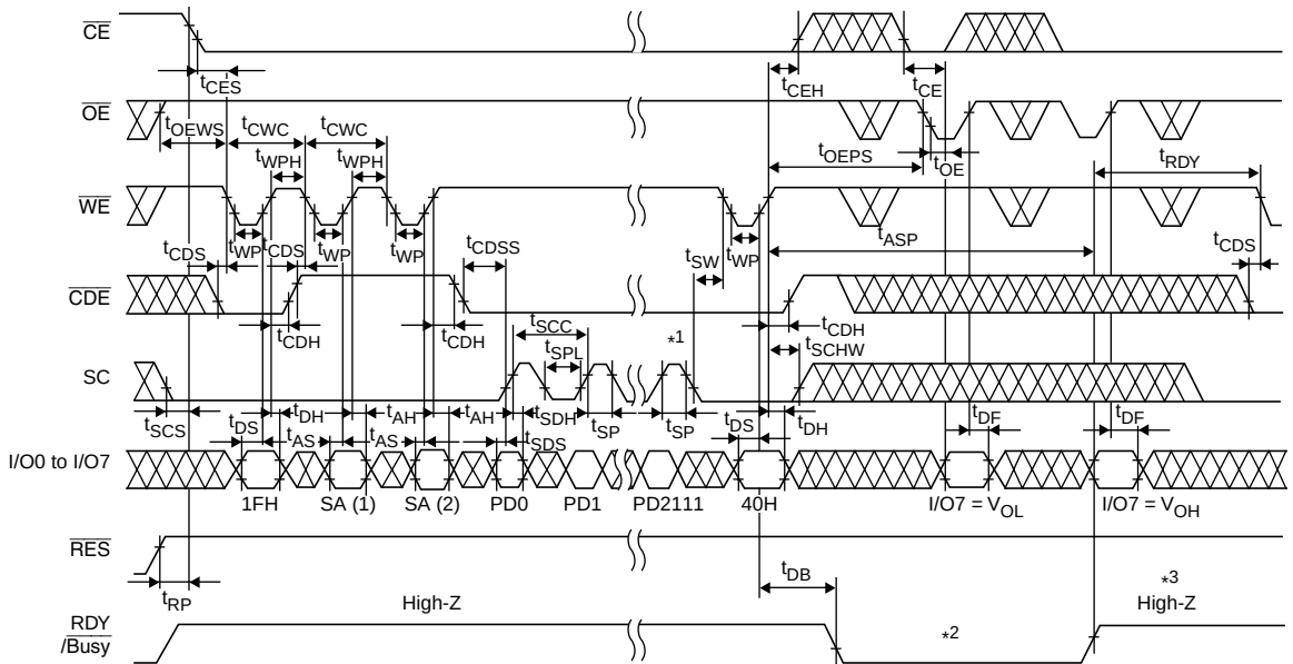
Program (2) and Status Data Polling Timing Waveform
