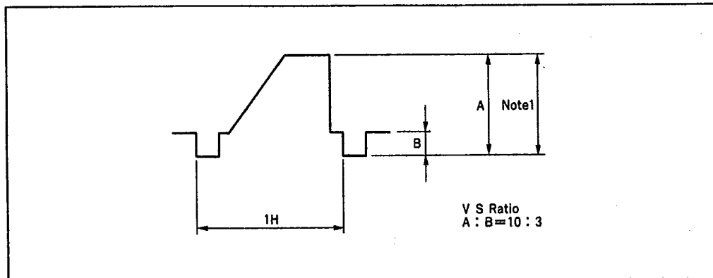
Video Signal-1
