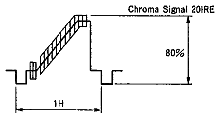
Video Signal-4
