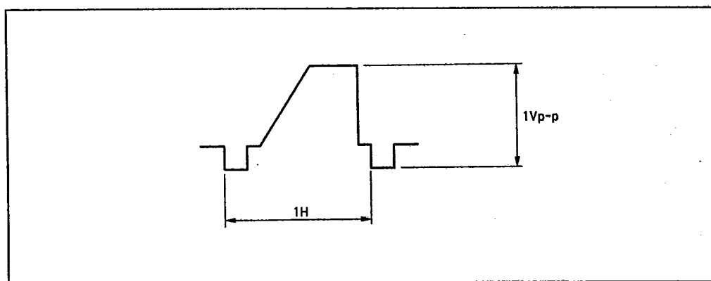
Video Signal-2
