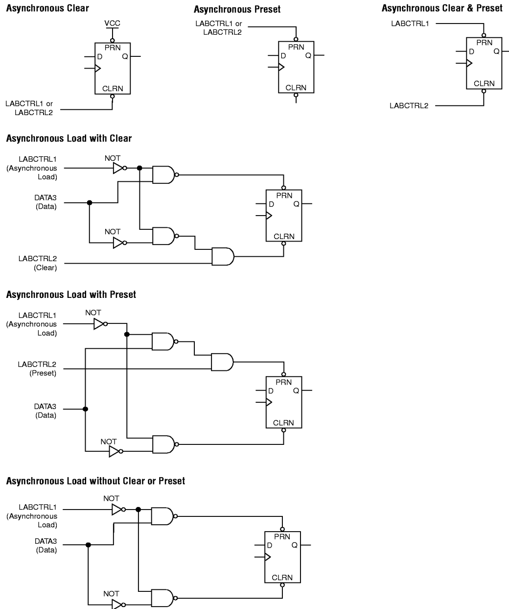
Figure 7. FLEX 8000 LE Asynchronous Clear & Preset Modes
