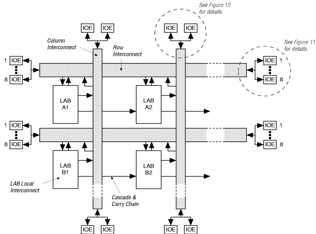
Figure 9. FLEX 8000 Device Interconnect Resources
