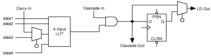
Figure 6. FLEX 8000 LE Operating Modes
