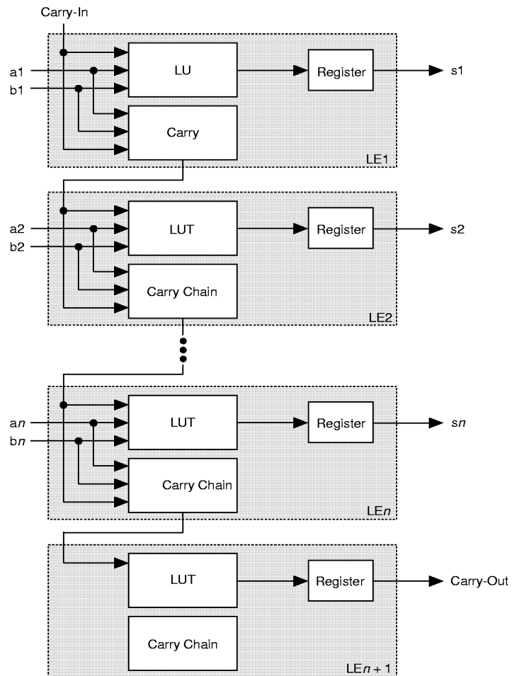
Figure 4. FLEX 8000 Carry Chain Operation
