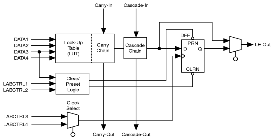
Figure 3. FLEX 8000 LE
