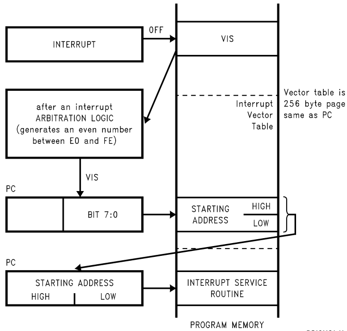
FIGURE 14. VIS Operation
