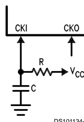
FIGURE 6. Crystal and R/C Oscillator Diagrams
