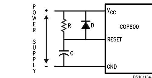
FIGURE 5. Recommended Reset Circuit
