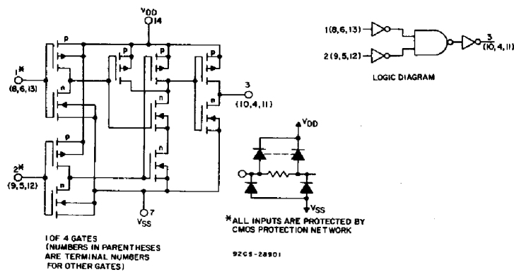
Fig. 5 - Schematic and logic diagrams for CD4001B.
