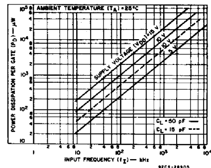
Fig. 2 - Typical power dissipation vs. frequency.
