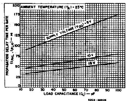
Fig. 11 - Typical propagation delay time vs. load capacitance.
