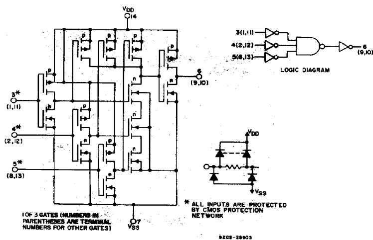
Fig. 7 - Schematic and logic diagrams for CD4025B.
