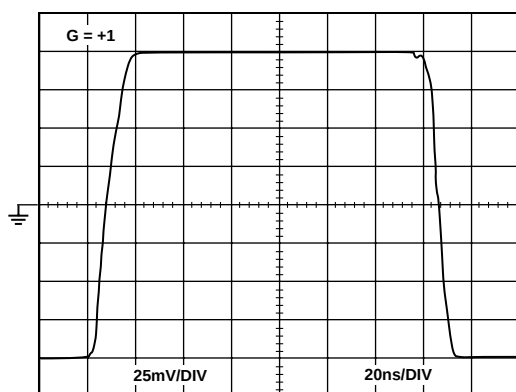
TPC 19. Small Signal Transient Response +5\text{ V} (See Test Circuit 1)
