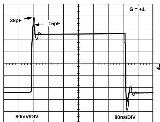
TPC 22. Small Signal Transient Response \pm 5\text{ V} (See Test Circuit 1)
