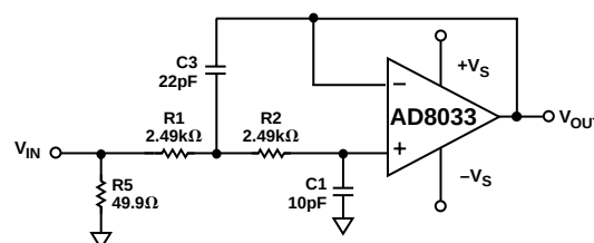
Figure 10. Two-Pole Butterworth Active Filter
