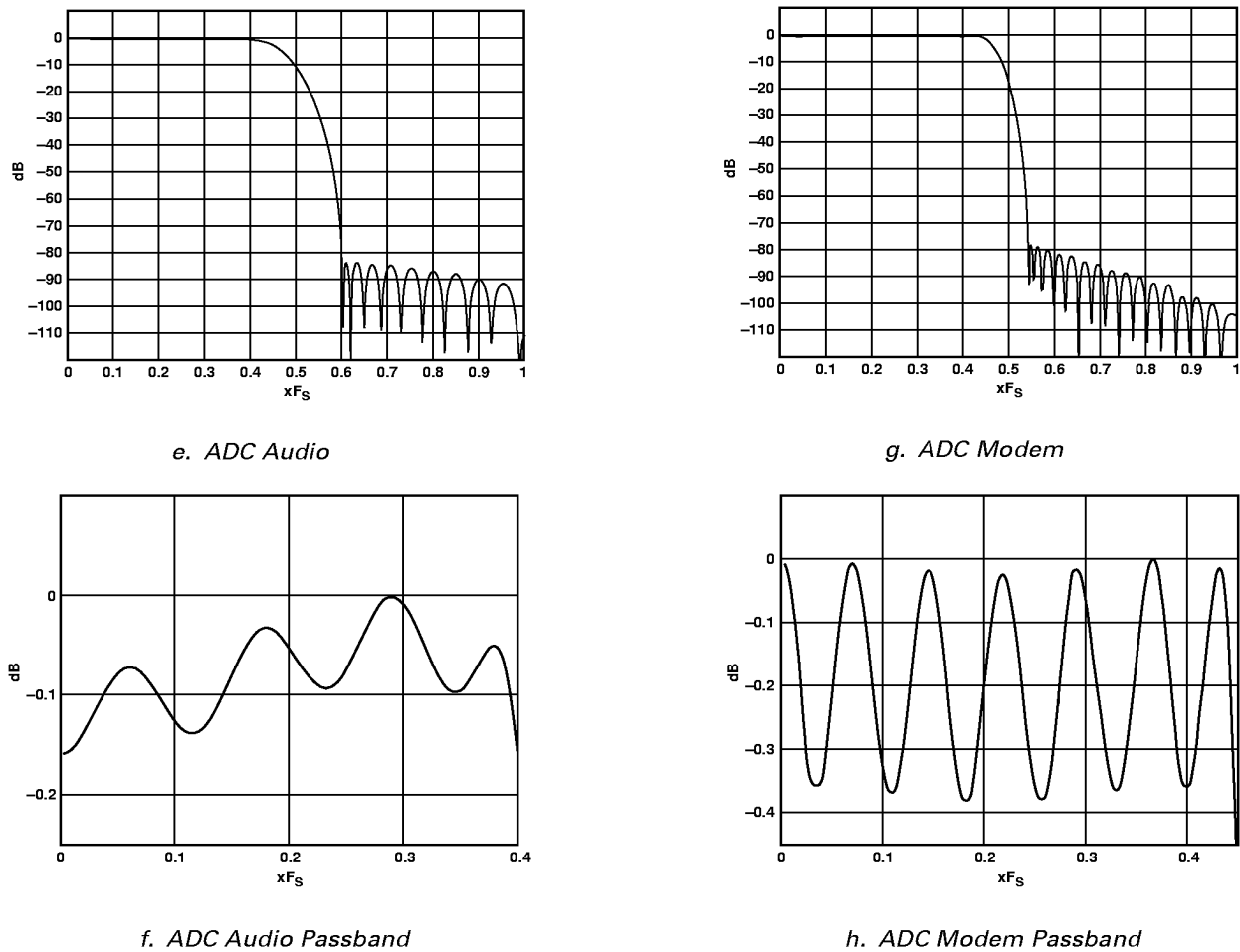
Figure 16. AD1815 Frequency Response Plots (Full-Scale Line-Level Input, 0 dB Gain). The Plots Do Not Reflect the Additional Benefits of the AD1815 Analog Filters. Out-of-Band Images Will Be Attenuated by an Additional 31.4 dB at 100 kHz.
