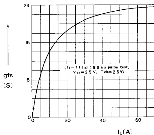
Typical Forward Transconductance vs. I_D
