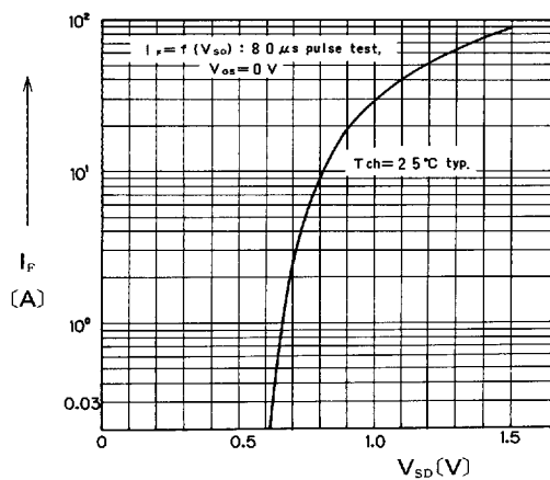
Forward Characteristics of Reverse Diode
