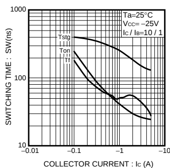
Fig.2 Switching Time
