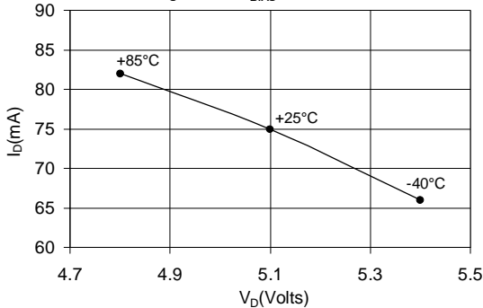
V_D vs. I_D over Temperature for fixed V_S = 8 \text{ V} , R_{BIAS} = 39 \text{ ohms} *
