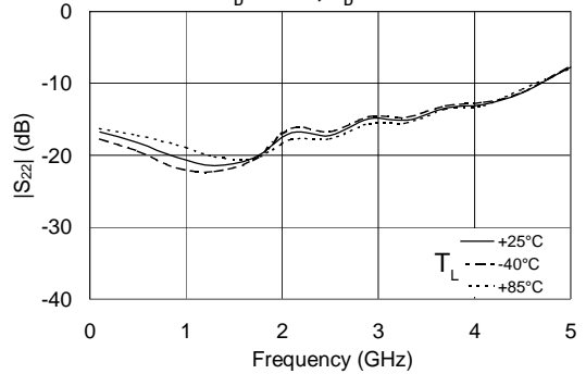
|S_{22}| vs. Frequency V_D = 5.1 \text{ V} , I_D = 75 \text{ mA}
