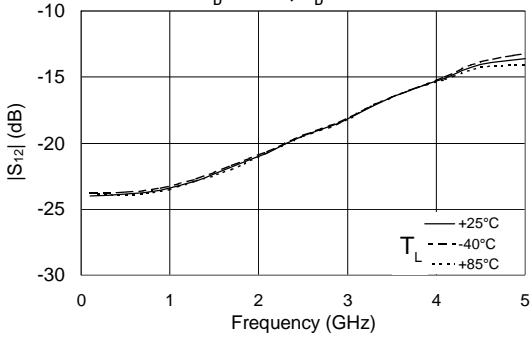
|S_{12}| vs. Frequency V_D = 5.1 \text{ V} , I_D = 75 \text{ mA}
