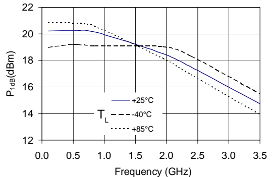
P 1dB vs. Frequency V_D = 5.1\text{ V}, I_D = 75\text{ mA}
