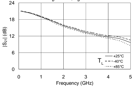
|S_{21}| vs. Frequency V_D = 5.1 \text{ V} , I_D = 75 \text{ mA}
