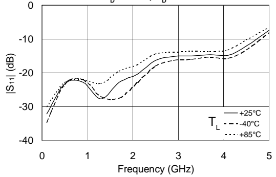
|S_{11}| vs. Frequency V_D = 5.1 \text{ V} , I_D = 75 \text{ mA}
