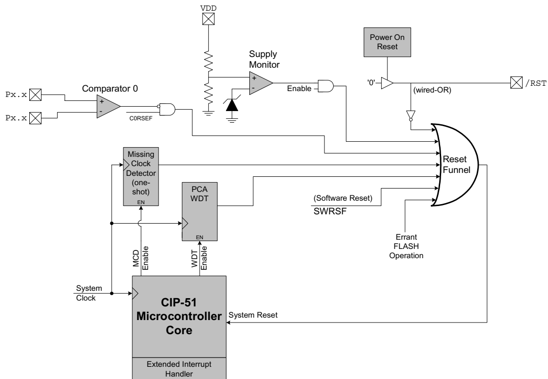
Figure 10.1. Reset Sources
