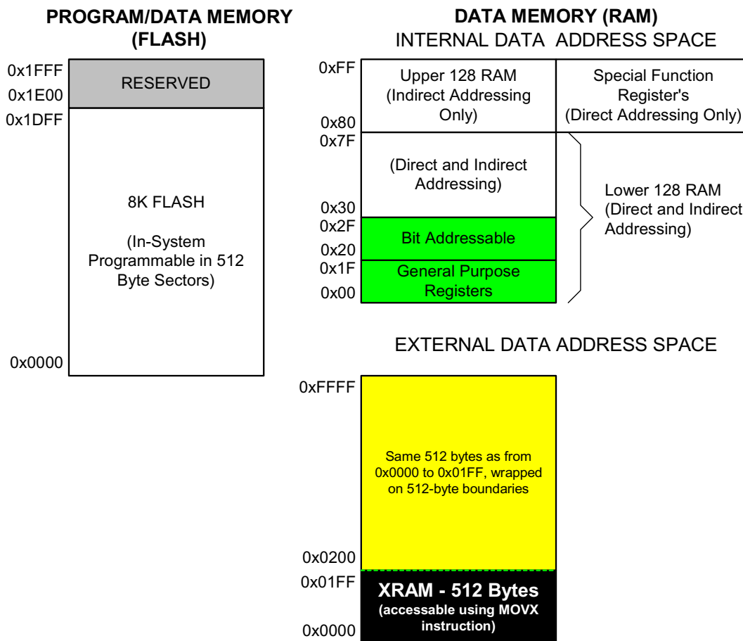
Figure 9.2. Memory Map
