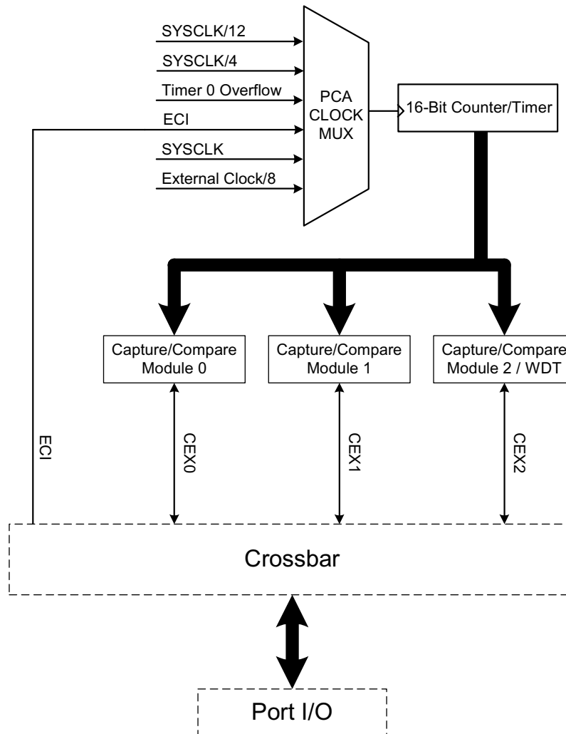
Figure 1.8. PCA Block Diagram
