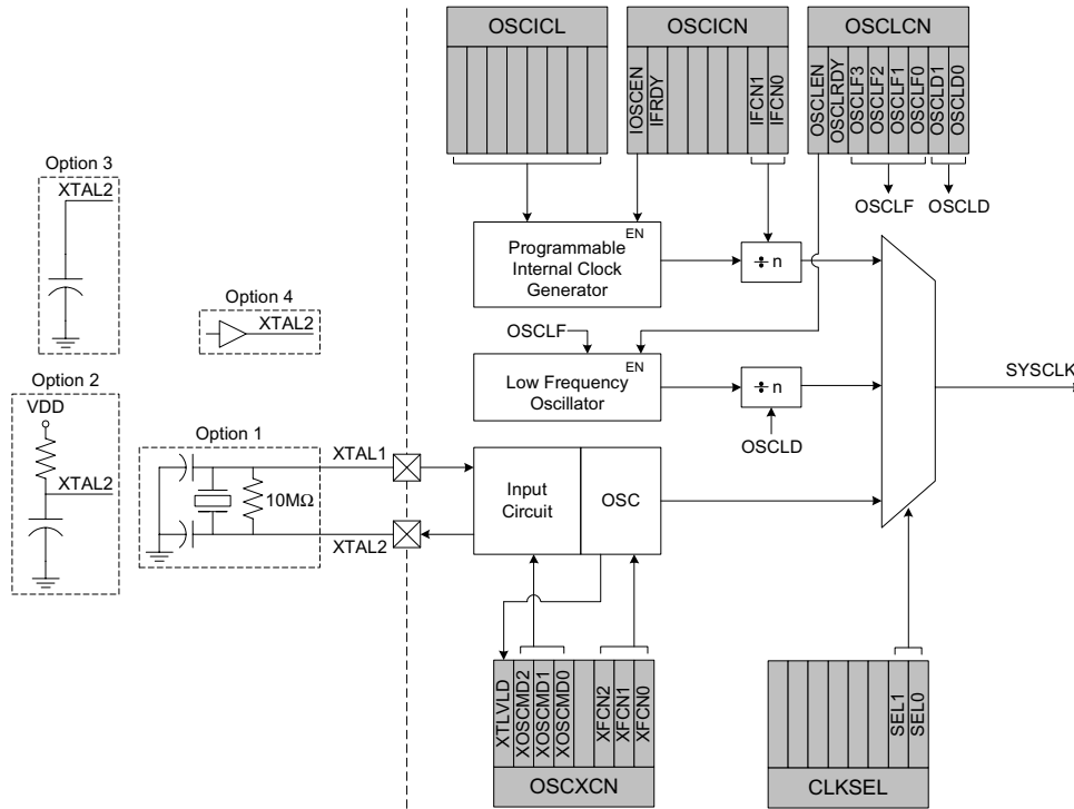
Figure 13.1. Oscillator Diagram
