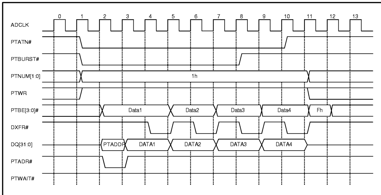
Active Mode PCI Write Showing a One Wait State Programmed Delay
