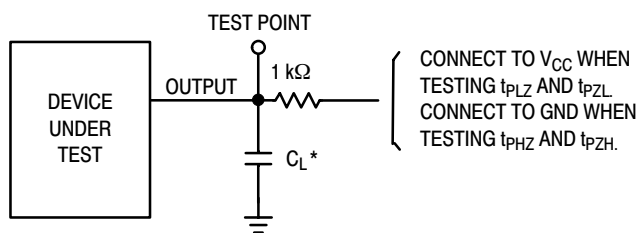
Figure 7. Test Circuit
