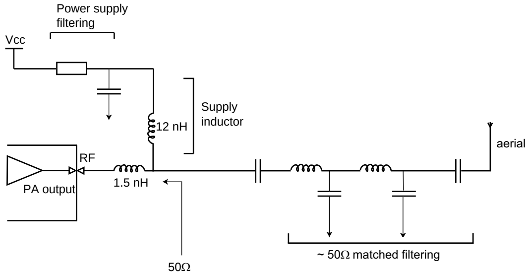
Figure 25. Output Matching at 868 MHz
