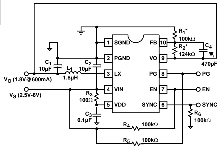
EL7530 TOP VIEW
