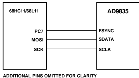
Figure 25. 68HC11/68L11-to-AD9835 Interface
