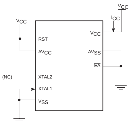
Figure 37. I_{CC} Test Condition, Power Down Mode All other pins are disconnected. V_{CC} = 2\text{V to } 5.5\text{V}
