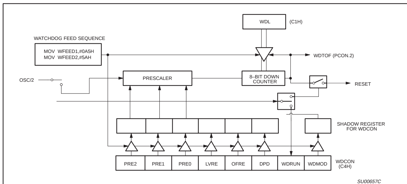
Figure 15. Watchdog Timer in 87C576 and 80C576 / 83C576 ( \overline{\text{EA}} = 0 )
