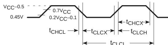
Figure 36. Clock Signal Waveform for I_{CC} Tests in Active and Idle Modes t_{CLCH} = t_{CHCL} = 5\text{ns}
