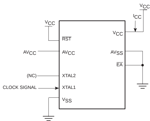
Figure 35. I_{CC} Test Condition, Idle Mode All other pins are disconnected
