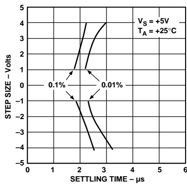
Figure 31. Settling Time vs. Step Size
