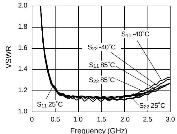
VSWR vs. Frequency Insertion Loss State
