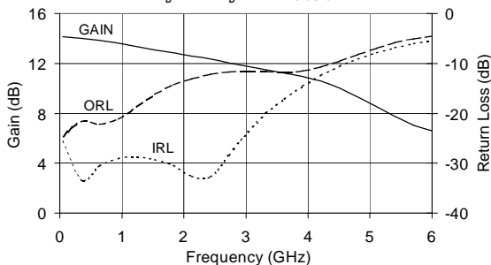
Gain & Return Loss vs. Frequency V_D = 3.2 \text{ V} , I_D = 45 \text{ mA} (Typ.)
