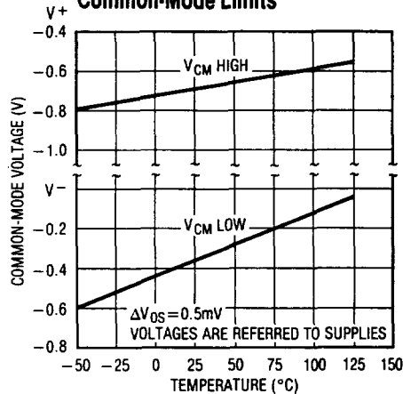
Common-Mode Limits
