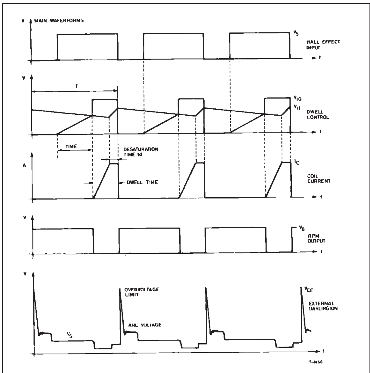
Figure 1 : Main Waveforms.
