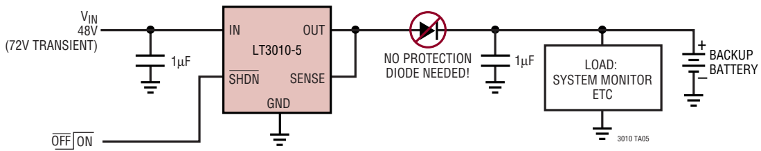
LT3010 Telecom Application
