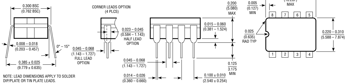
J8 Package 8-Lead Ceramic Dip
