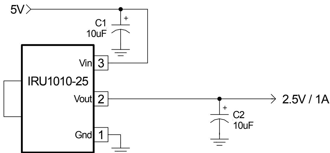
Figure 1 - Typical application of IRU1010-25 in a 5V to 2.5V regulator
