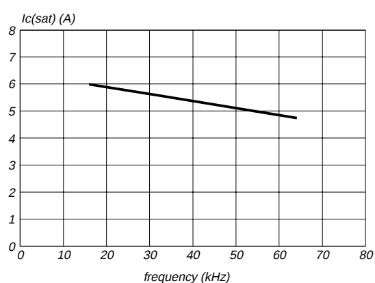
Fig.14. I_{C\text{sat}} during normal running vs. frequency of operation for optimum performance
