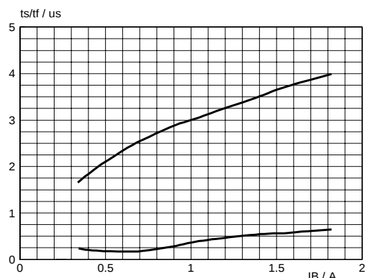
Fig.9. Typical collector storage and fall time. t_s = f(I_B) ; t_f = f(I_B) ; I_C = 4.5 \text{ A} ; T_j = 85^\circ\text{C} ; f = 56 \text{ kHz}
