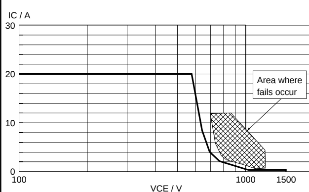
Fig.13. Reverse bias safe operating area. T_j \leq T_{j\text{max}}
