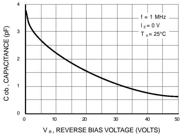
Figure 4. Output Capacitance
