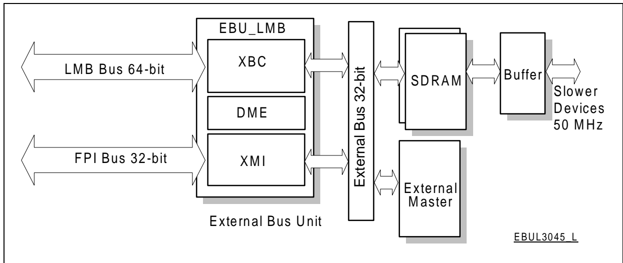
Figure 4 EBU_LMB block diagram
