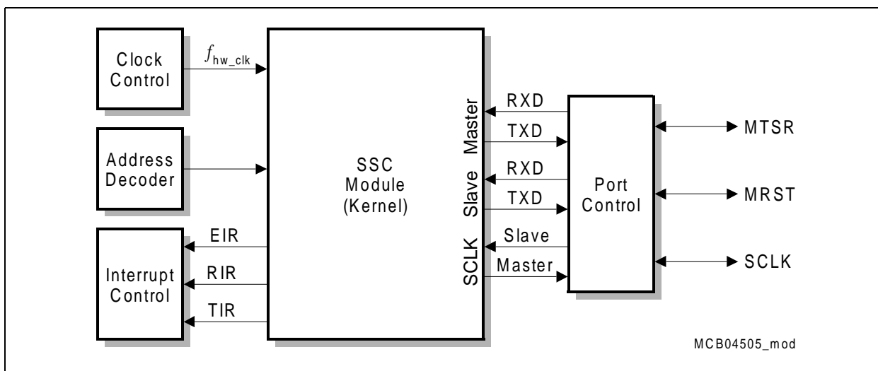
Figure 7 General Block Diagram of the SSC Interface
