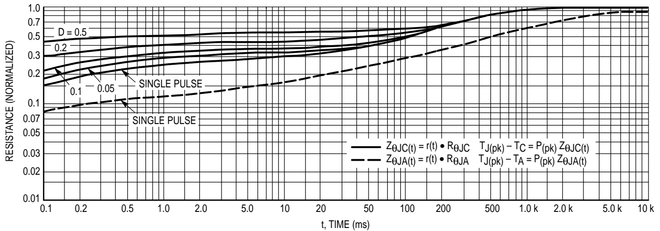
Figure 9. Thermal Response
