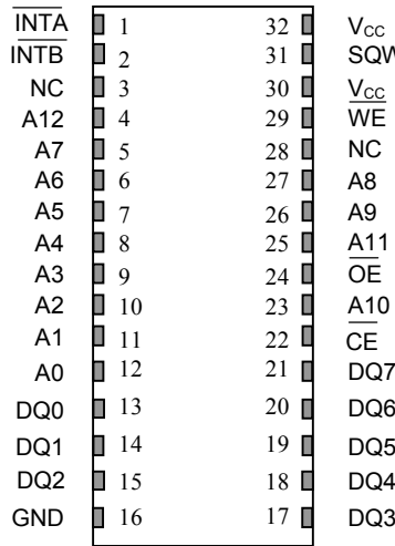
DS1386 8k x 8 32-Pin Encapsulated Package
