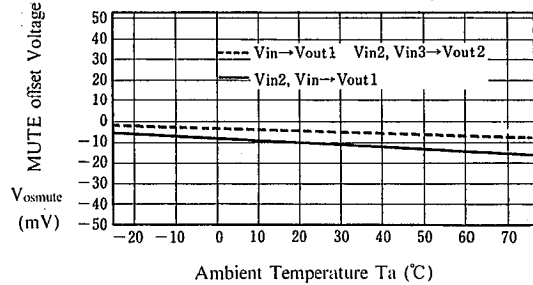
MUTE offset Voltage vs. Temperature
