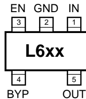
MIC5252-x.xBM5 SOT-23-5 (M5) (Top View)
