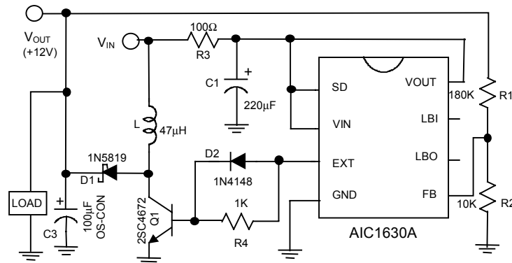
Fig. 2 12V Output Step-Up Converter for Flash Memory
