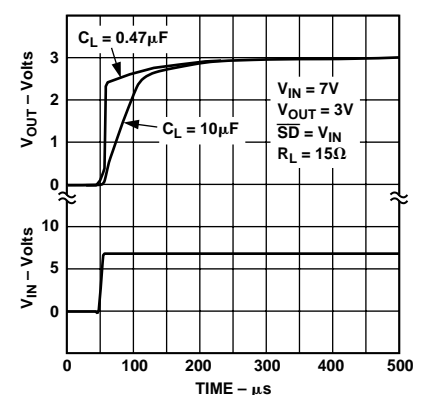
Figure 10. Power-Up Response
