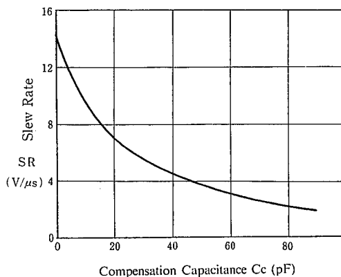
Slew Rate
