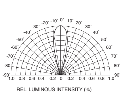
Fig.4 Radiation Diagram
